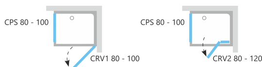
CRV1/CRV2 CPS zuhanykabin
